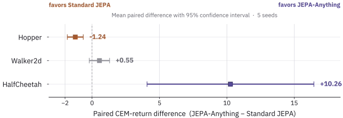
Figure 6 | Capacity-matched continuous-control planning. Squares show the mean paired CEM-return difference between JEPA-Anything and standard JEPA over five training seeds; error bars show 95% confidence intervals. Positive values favor JEPA-Anything.
