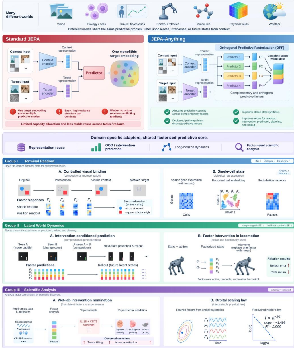
Figure 1 | Overview of JEPA-Anything. Upper section: Diverse domains share the same predictive problem: inferring unobserved, intervened, or future states from context. Standard JEPA mixes multiple predictive modes in a monolithic target embedding. In contrast, JEPA-Anything uses orthogonal predictive factorization (OPF) to allocate predictive capacity across complementary, orthogonal factors, each with a dedicated predictor, and synthesize a complete latent world state. The shared factorized core supports representation reuse, out-of-distribution and intervention prediction, long-horizon dynamics, and factor-level scientific analysis. Lower section: Three evaluation groups illustrate these capabilities. Group I (terminal readout) examines controlled visual binding and single-cell state representations. Group II (latent world dynamics) evaluates intervention-conditioned prediction and factor intervention in locomotion. Group III (scientific analysis) investigates wet-lab intervention nomination and the recovery of an orbital scaling law. Within each group, experiments A and B are arranged from left to right.
