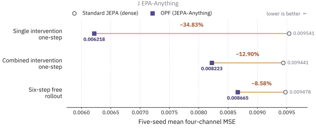
Figure 4 | Intervention-conditioned prediction and free rollout on CITRIS Interventional Pong. Lower four-channel MSE is better. Points show means over five paired seeds; annotations give the reduction computed from the reported means.
